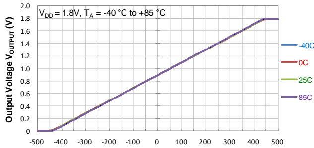
Output Voltage vs Magnetic Flux Density
