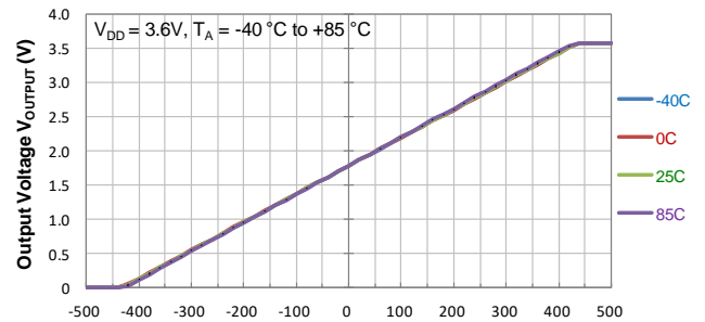
Output Voltage vs Magnetic Flux Density
