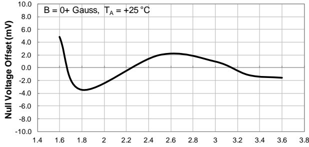
Supply Voltage (V) Null Voltage Offset vs Supply Voltage
