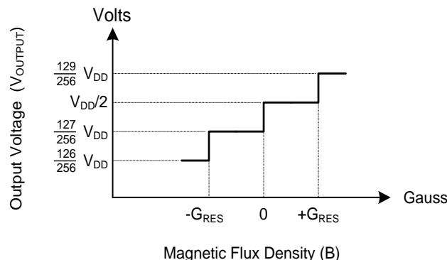
Transfer Curve Near 0 Gauss
