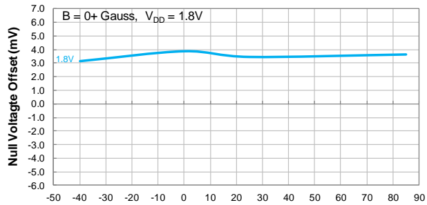
Temperature (°C) Null Voltage Offset vs Temperature
