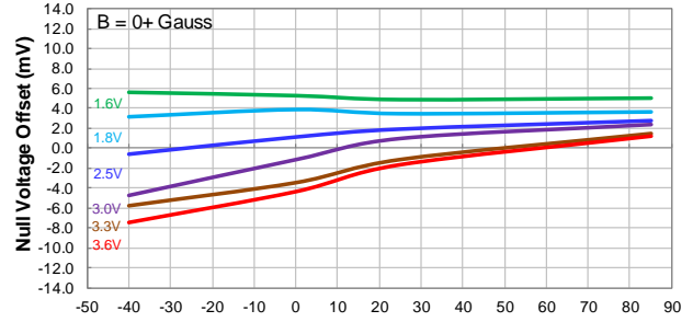
Temperature (°C) Null Voltage Offset vs Temperature
